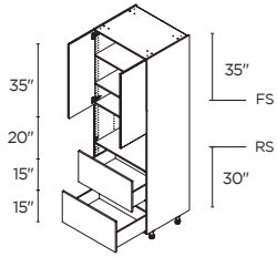
MICROWAVE 1 2 DOORS / 2 DRAWERS 30" | TM2D3089.5
