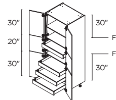
6 DOORS / 4 INNER DRAWERS 30" | T302484.514
