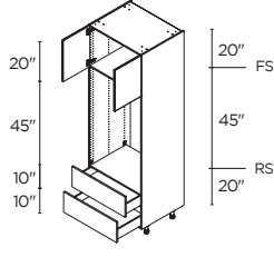
MICRO/WALL OVEN 2 2 DOORS / 2 DRAWERS 30" | TMO2DA3089.5
