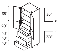
4 DOORS / 3 DRAWERS / 2 INNER DRAWERS 30" | T3DA302489.512
