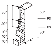
2 DOORS / 3 DRAWERS / 2 INNER DRAWERS 15" | T3DA152489.512(L/R) 18" | T3DA182489.512(L/R) 24" | T3DA242489.512(L/R)
