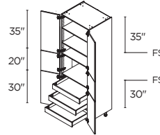
6 DOORS / 3 INNER DRAWERS 30" | T302489.513
