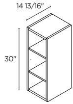
WALL OPEN SHELF 9" | WOS930
