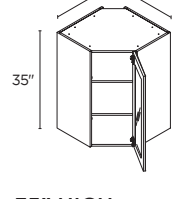
35" HIGH 1 GLASS DOOR* 24" | WAG2435(L/R)
