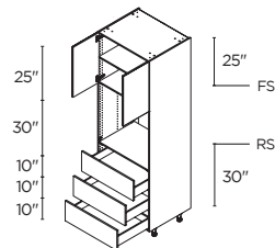
SINGLE OVEN 3 2 DOORS / 3 DRAWERS 30" | TO3DA3089.5
