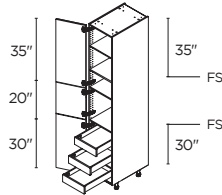
3 DOORS / 3 INNER DRAWERS 15" | T152489.513(L/R) 18" | T182489.513(L/R) 24" | T242489.513(L/R)
