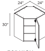
30" HIGH 1 DOOR 24" | WA2430(L/R)
